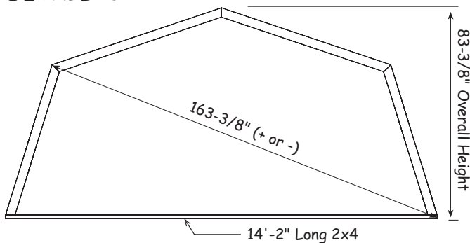
DETAIL 'C'
