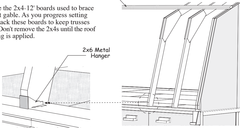
2x4-12' Board
