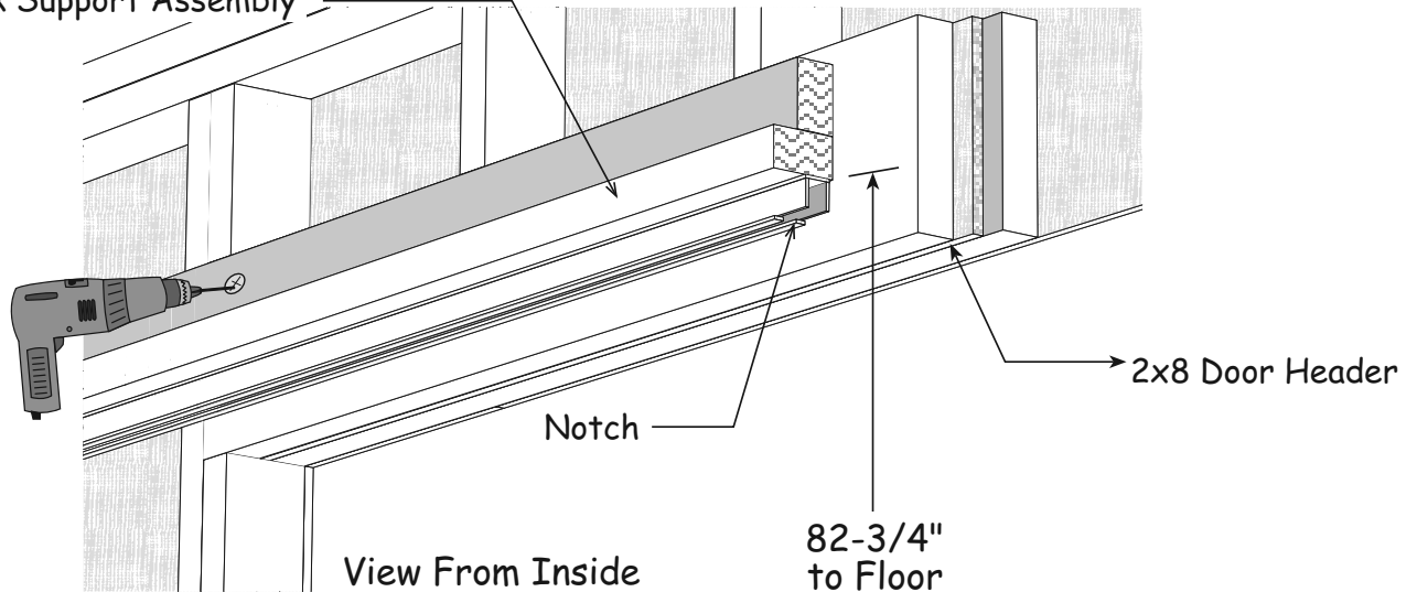
2x3 Track Support Assembly
