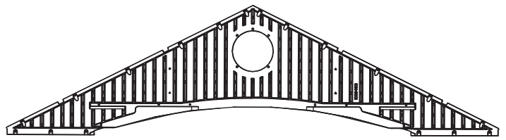
Side Entry Gable Assembly (x1)
