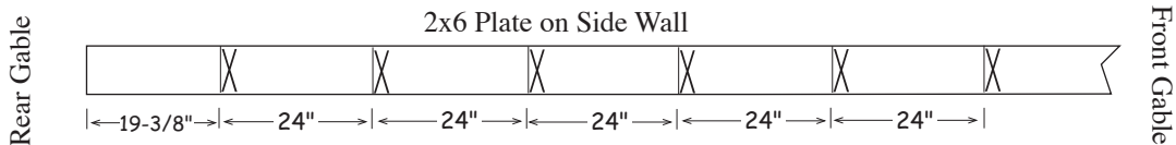
Detail 'A'
