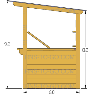
END VIEW - CLOSED SCALE 1"=1'-0"
