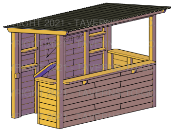
FRONT ISOMETRIC VIEW
