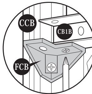
Fig.2: Use (S1) screw. Fix (CB1B) to (FCB)
