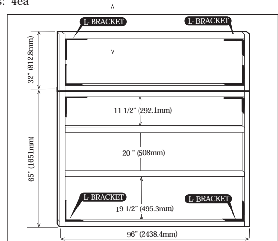
Foundation Structure
